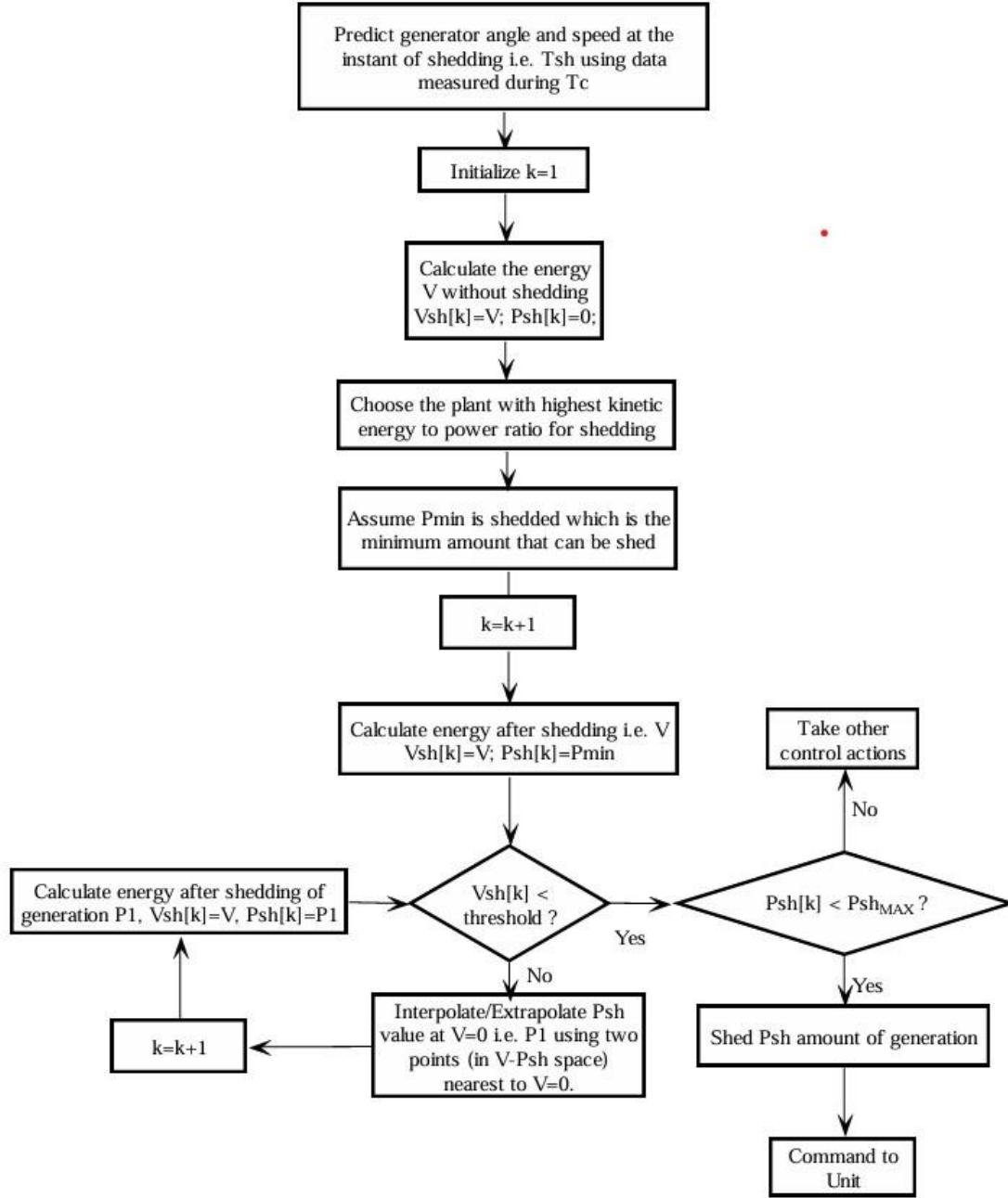
Fig. 1: Flowchart for generation shedding
